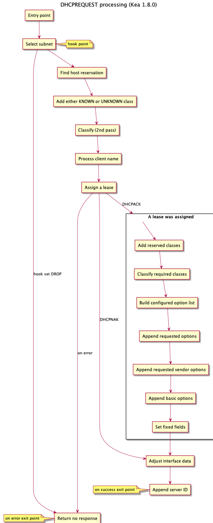
Fig. 3: DHCPREQUEST processing
